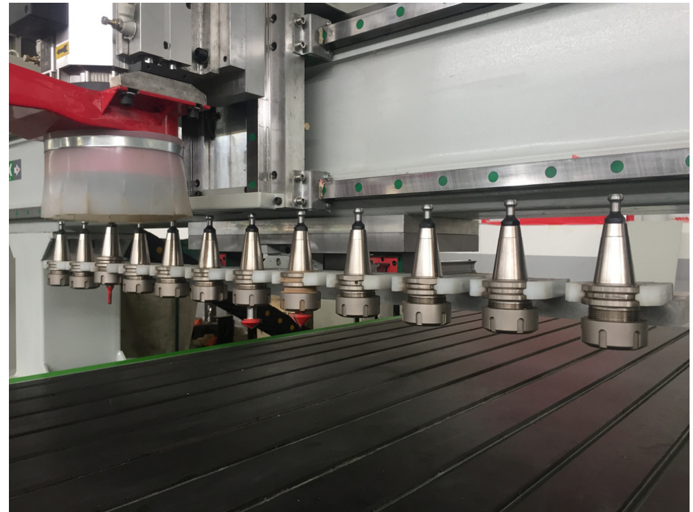
12-Tools Linear ATC
