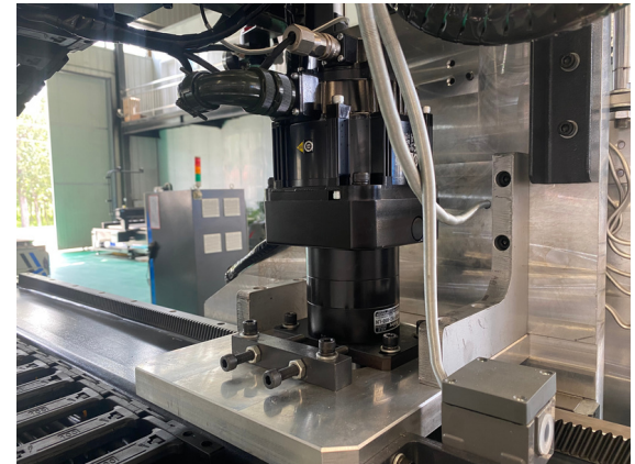
Optional HSD 9-Tools Drill Bank
